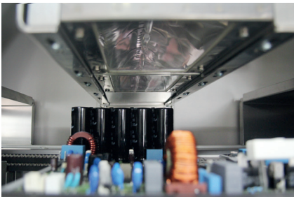
High-performance lamps in the RDS 1200 UV for drying all UV-hardened coatings
